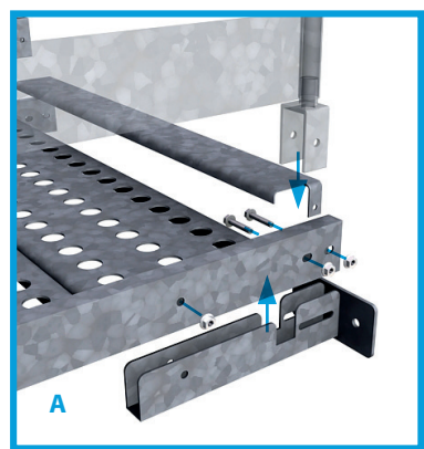
RACCORD MURAL ESCALIER PALIER
